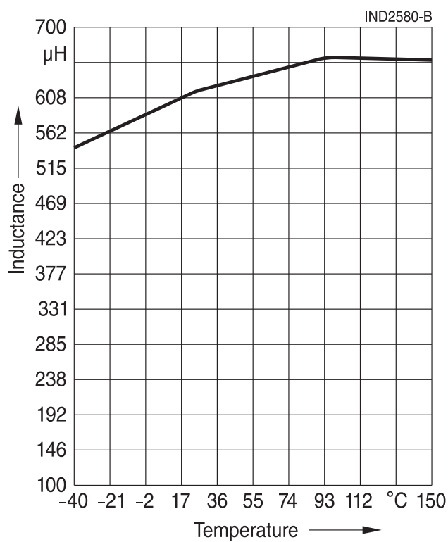
Typical inductance vs. temperature graph
