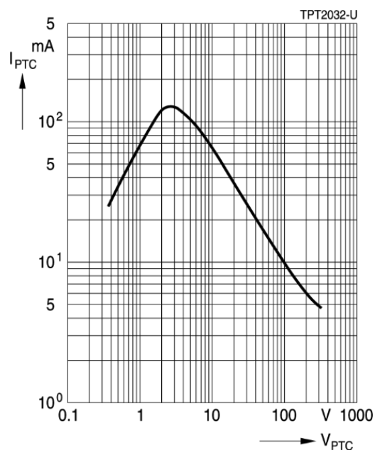
PTC current I_{PTC} versus PTC voltage V_{PTC} (measured at 25 °C in still air)
