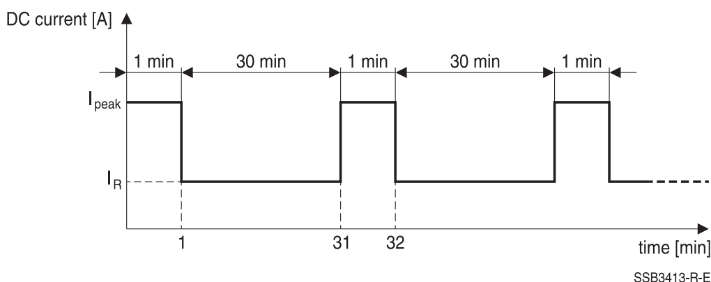
Fig.1: Permissible time lapse for peak current 650 A DC
