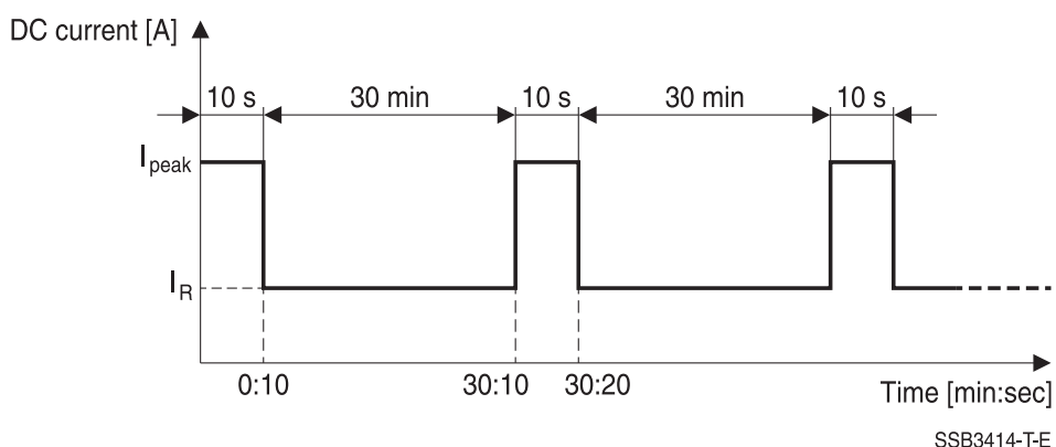
Fig 2: Permissible time lapse for peak current 1000 A DC
