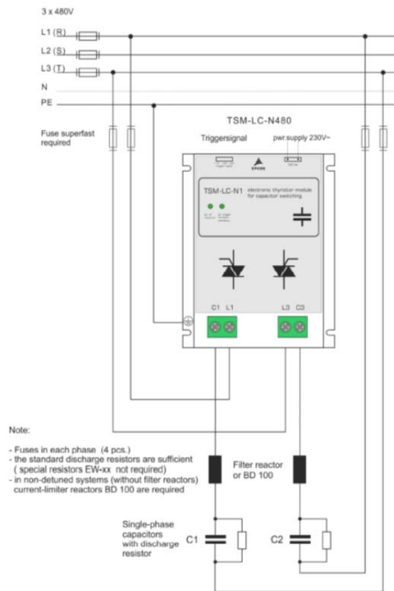
Pict.2: Connection diagram, two phase load
