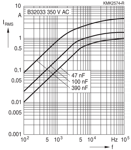
Lead spacing 22.5 mm
