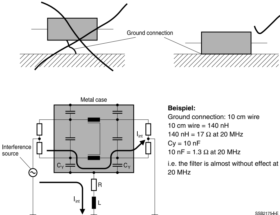
Figure 26 Effects of incorrect filter mounting
