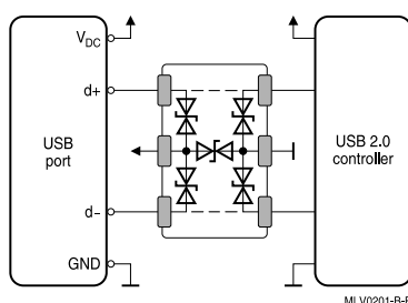
Figure 8 USB 2.0 line protection with special array CDA3C05GTH
