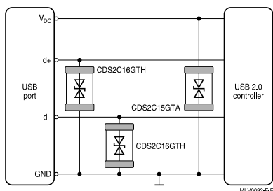
Figure 7 USB 2.0 line protection with single CeraDiodes
