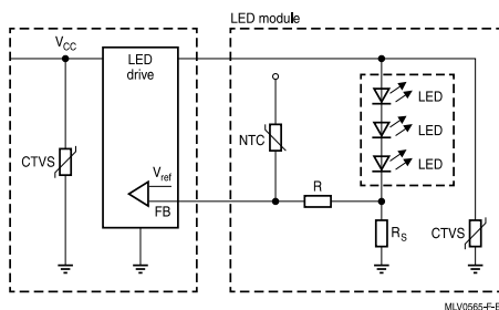
Figure 6 LED circuit with multilayer varistors and temperature control
