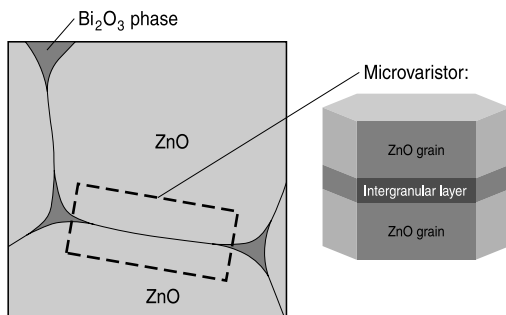
Figure 11 Microstructure of CTVS
