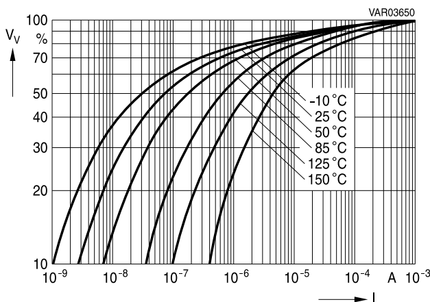
Figure 28 Typical temperature dependence of the V/I characteristic
