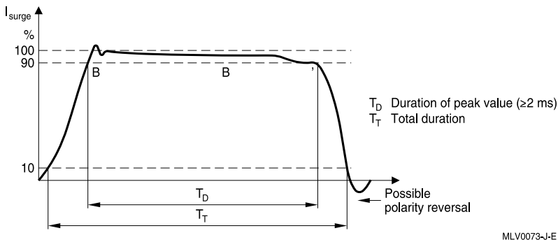
Figure 24 2 ms surge current waveform to IEC 62475 standard
