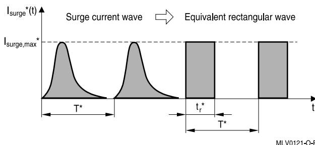
Figure 1 Rectangular wave method
