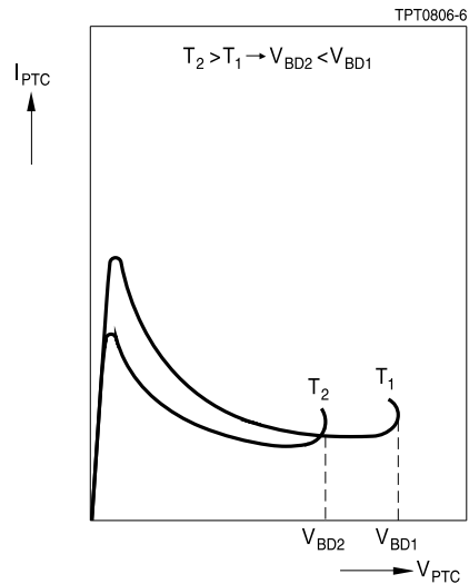
Figure 9 Influence of the ambient temperature on the I/V characteristic
