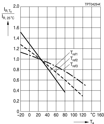
Figure 4 Standardized rated current I_R versus ambient temperature T_A (measured in still air) Parameter: T_{ref1} < T_{ref2} < T_{ref3}
