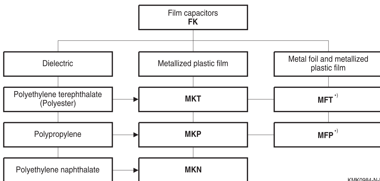
Figure 1 Classification of film capacitors in DIN EN 60062:2005
