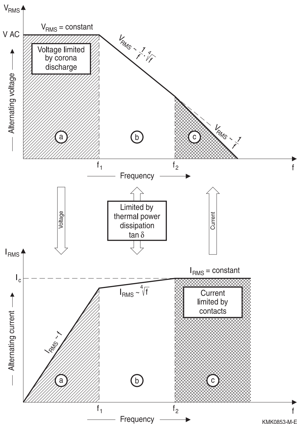
Figure 22 Alternating voltage and alternating current load limits
