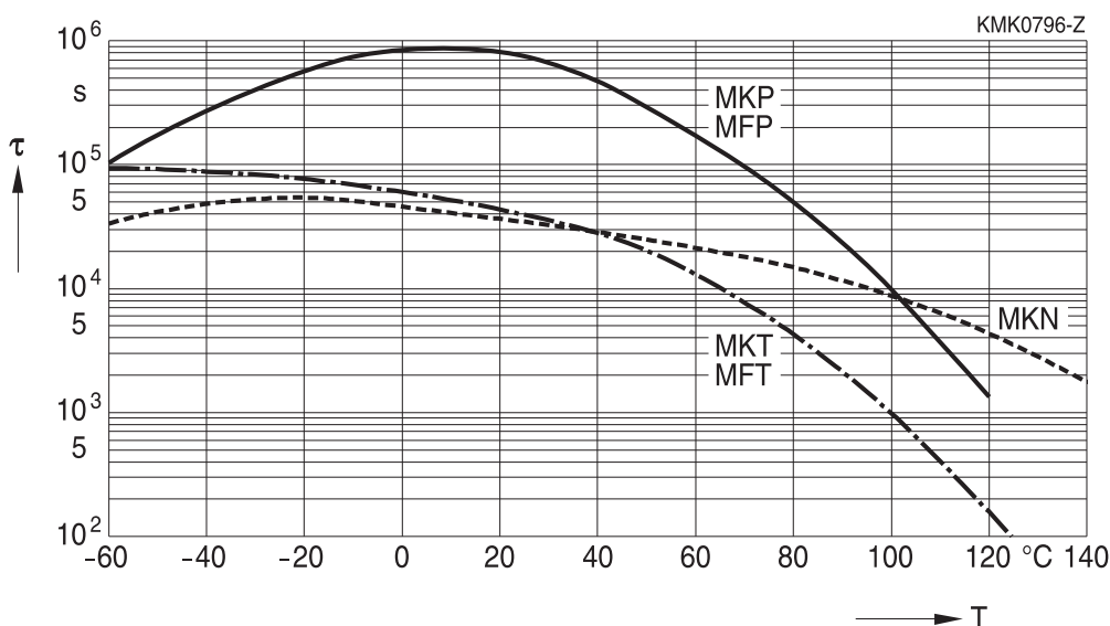
Figure 18 Insulation as self-discharge time constant \tau ( = R_{ins} \cdot C_R ) in s ( \triangleq M\Omega \cdot \mu F ) vs. temperature T (typical values)
