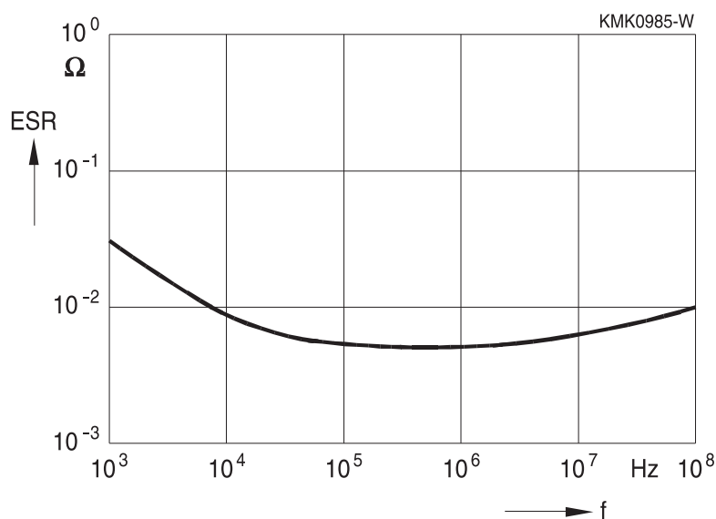
Figure 17 ESR vs. frequency for an MKT capacitor
