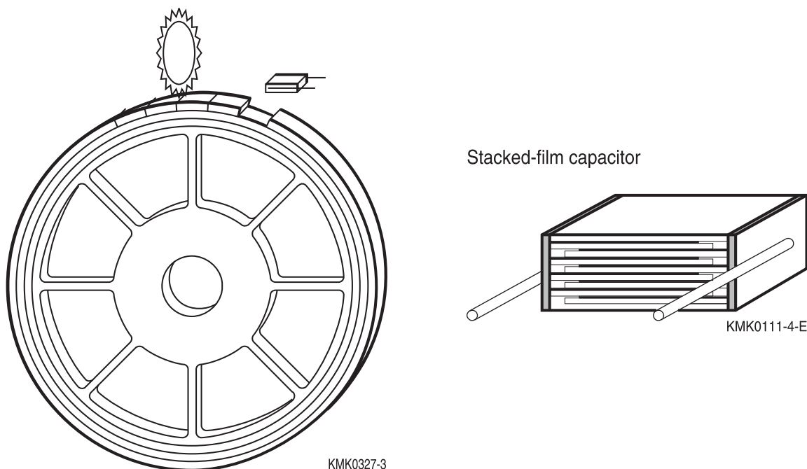
Figure 5 Stacked-film production technology
