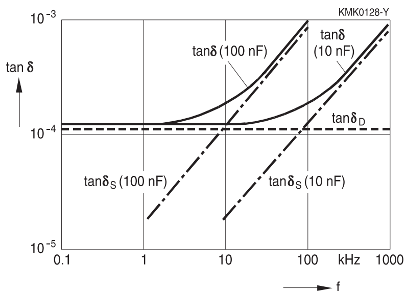
Figure 15 Dissipation factor \tan \delta vs. measuring frequency f (schematic representation using two polypropylene capacitors of different capacitance as examples)
