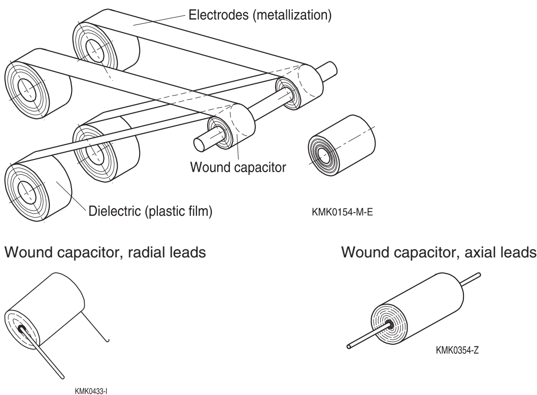
Figure 4 Conventional production process in wound technology
