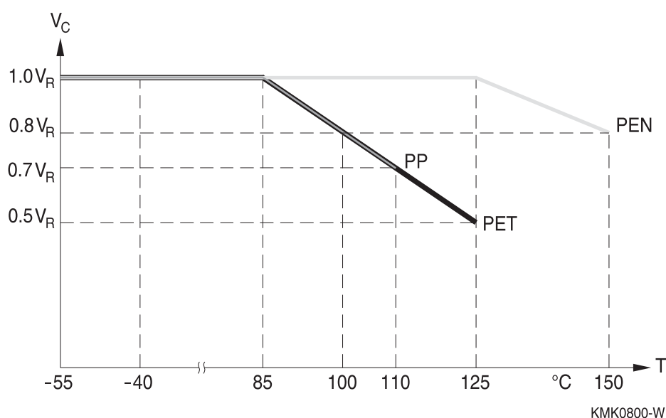
Figure 21 Maximum permissible continuous voltage vs. temperature T
