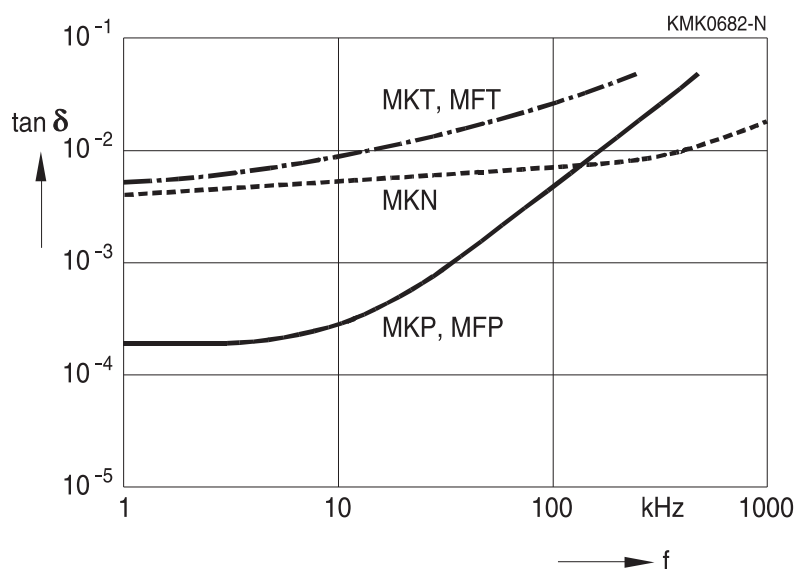
Figure 14 Frequency dependence of dissipation factor \tan \delta , e.g. for C_R = 0.10 \mu\text{F} (typical behavior)
