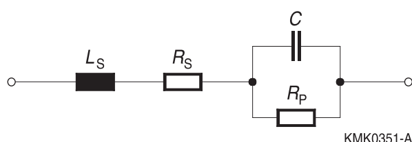
Figure 8 Real capacitor model
