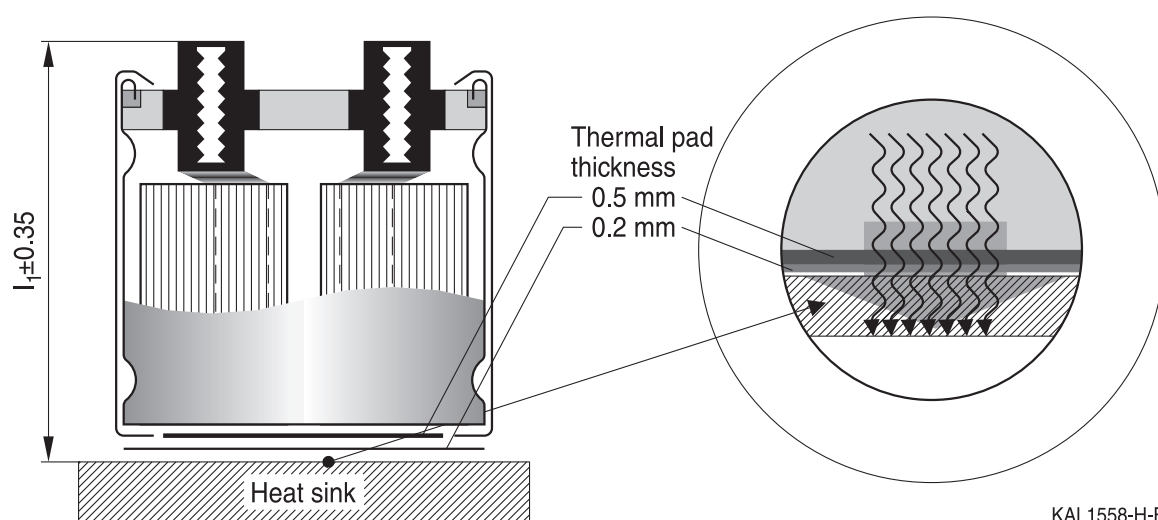
Figure 16 Heat-sink mounting for capacitors with screw terminals
