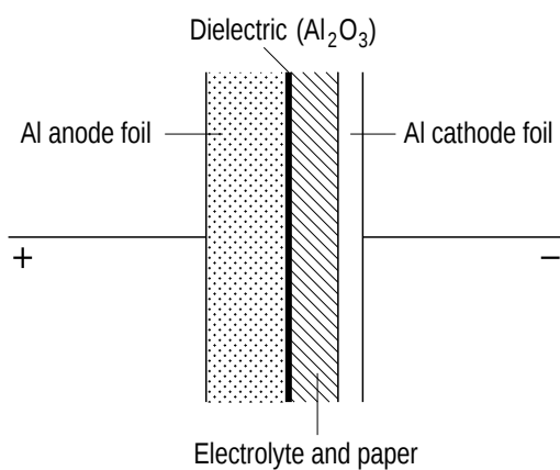
Figure 1 Basic construction of an aluminum electrolytic capacitor
