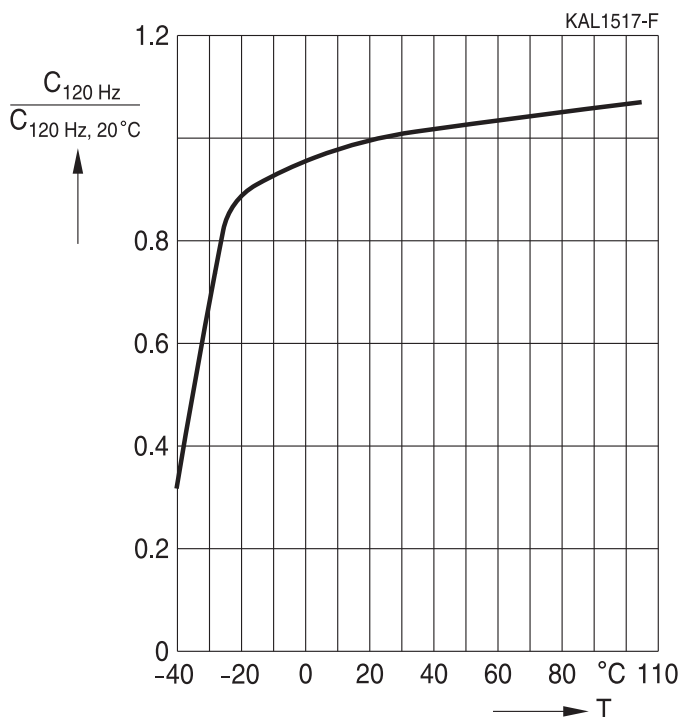
Figure 7 Example of temperature dependence of capacitance C
