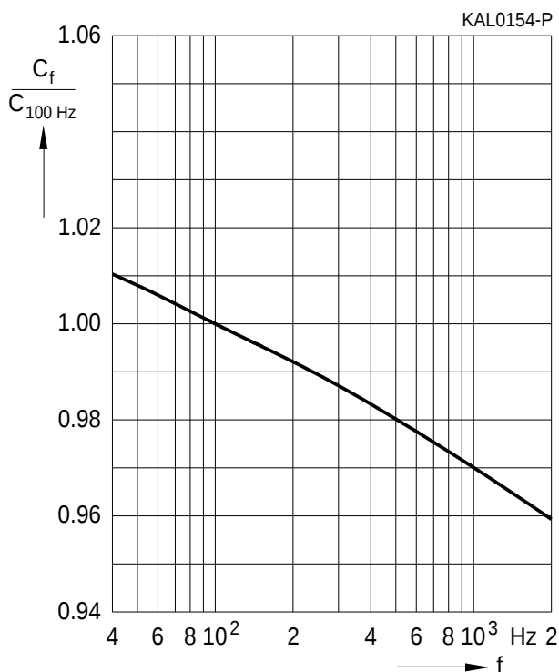
Figure 8 Capacitance C versus frequency f Typical behavior
