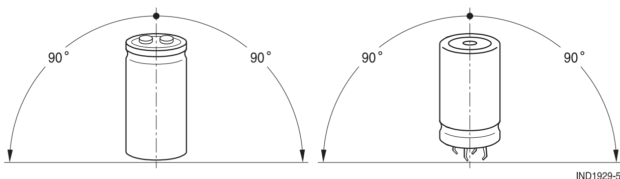
Figure 23 Recommended range of mounting positions
