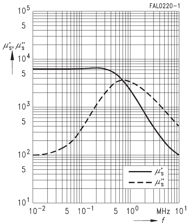
Complex permeability versus frequency (measured on R16 toroids, \hat{B} \leq 0.25 mT)
