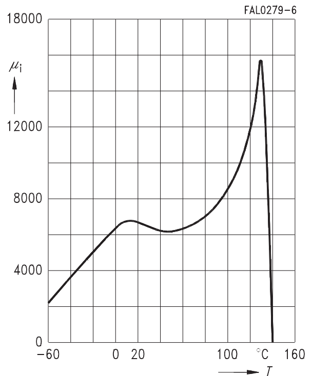
Initial permeability \mu_i versus temperature (measured on R22 toroids, \hat{B} \leq 0.25 mT)
