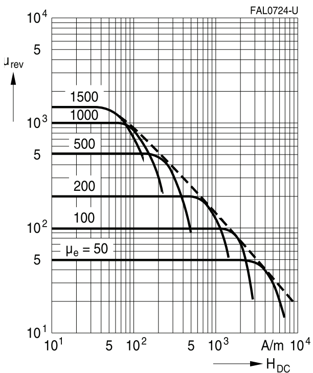
DC magnetic bias (measured on ETD cores, typical values) ( \hat{B} \leq 0.25 \text{ mT} , f = 10 \text{ kHz} , T = 25 \text{ }^\circ\text{C} )
