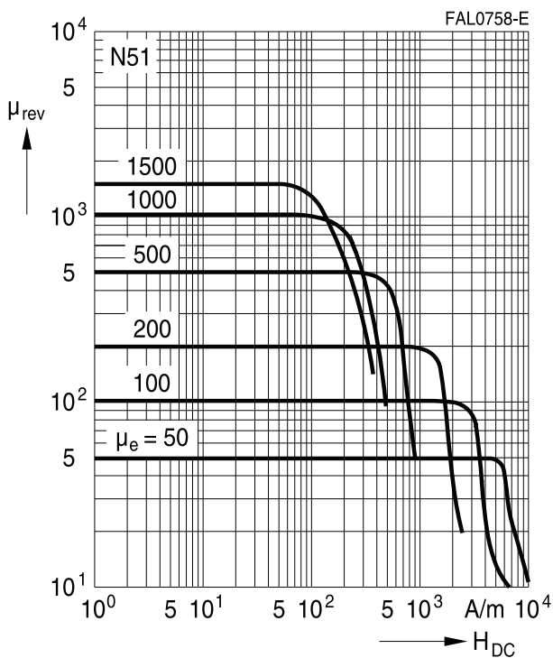
DC magnetic bias measured on E cores ( \hat{B} \leq 0.25 mT, f = 10 kHz, T = 25 °C)
