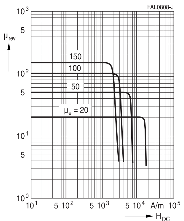
DC Magnetic bias measured on EQ30 cores ( \hat{B} \leq 0.25 mT, f = 10 kHz, T = 100 °C)
