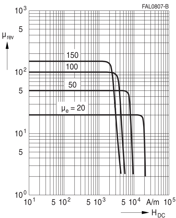
DC Magnetic bias measured on EQ30 cores ( \hat{B} \leq 0.25 mT, f = 10 kHz, T = 25 °C)
