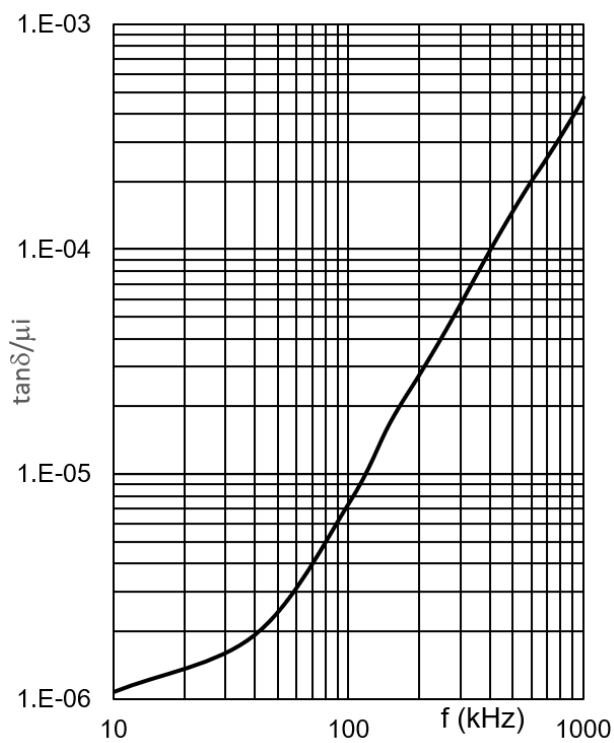
Relative loss factor versus frequency (measured on R12.5 toroids, B \leq 0.25 mT)
