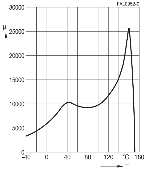
Initial permeability \mu_i versus temperature (measured on R12.5 toroids, B \leq 0.25 mT)
