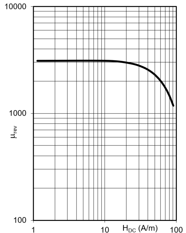
DC magnetic bias measured on RM10 cores (typical values) ( B \leq 0.25 mT, f = 10 kHz, T = 25 °C)
