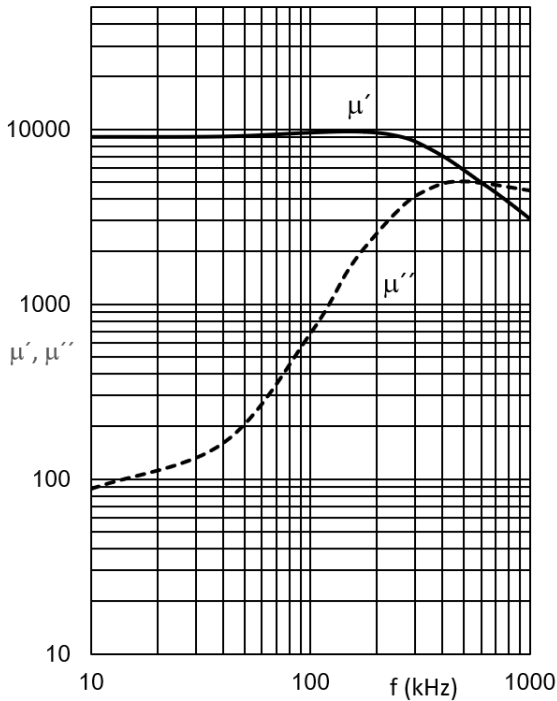
Complex permeability versus frequency (measured on R12.5 toroids, B \leq 0.25 mT)
