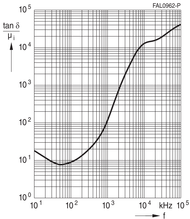
Relative core loss factor versus frequency (measured on R34 toroids, \hat{B} \leq 0.25 mT)
