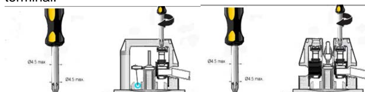
Figure 5: Fixing the supply cable.
