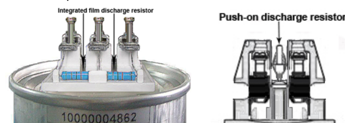
Figure 6: Different discharge resistors
