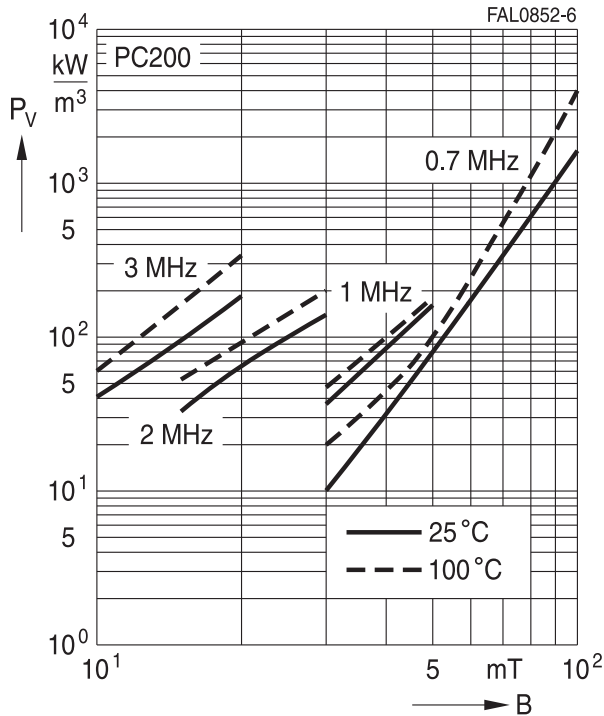
Relative core losses versus AC field flux density (measured on R20 toroids)
