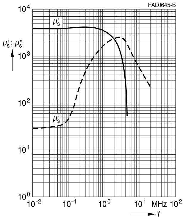
Complex permeability versus frequency (measured on R17 toroids, \hat{B} \leq 0.25 mT)
