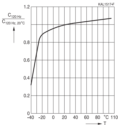
Figure 22 Temperature characteristics of capacitance C Typical behavior
