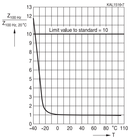
Figure 21 Temperature characteristics of impedance Z Typical behavior
