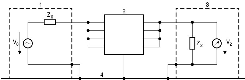
Figure 15 Asymmetrical measurement (according to EN 55017, Figure 5)
