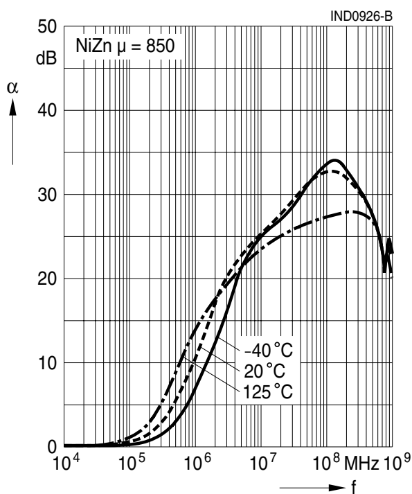
Figure 6 Insertion loss \alpha (common-mode) measured on B82793S0513N201
