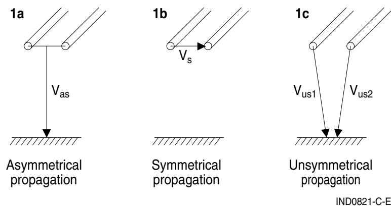
Figure 1 Propagation modes
